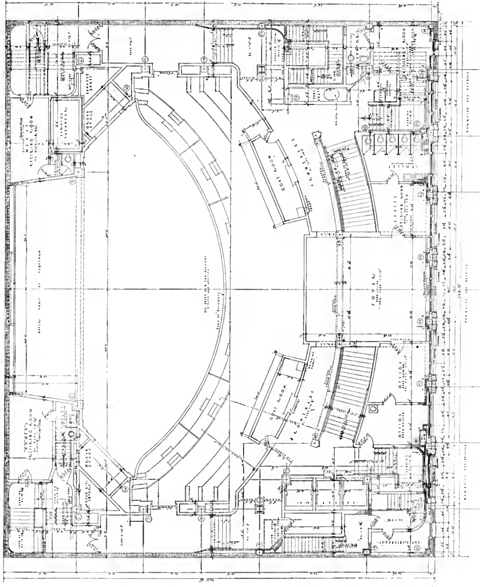
BALCONY MEZZANINE FLOOR PLAN THE TOWN HALL, NEW YORK CITY McKIM, MEAD & WHITE, ARCHITECTS
